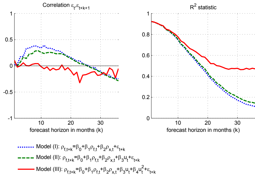
Figure 5: Diagnostic statistics.
