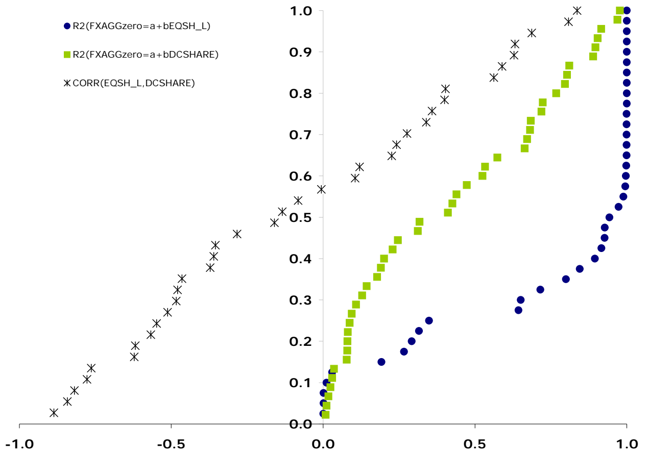
Figure 3: Decomposition FX^{AGG,zero} = EQSH_L + DCSHARE . Cross-country distribution of statistics.
