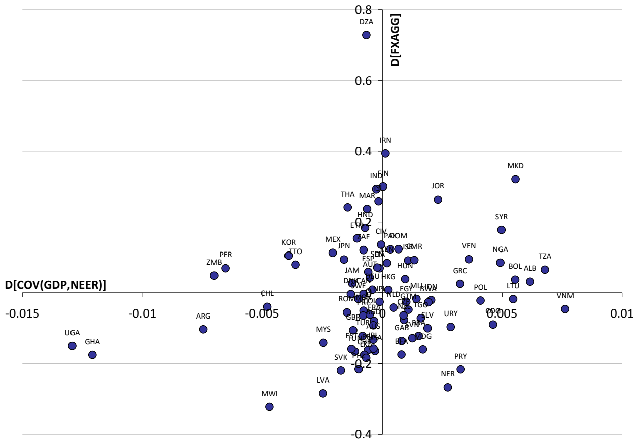
Figure 6: Scatter of Partial Relation between \Delta\text{COV}(\text{GDP}, \text{NEER}) and \Delta\text{FX}^{\text{AGG}} .
