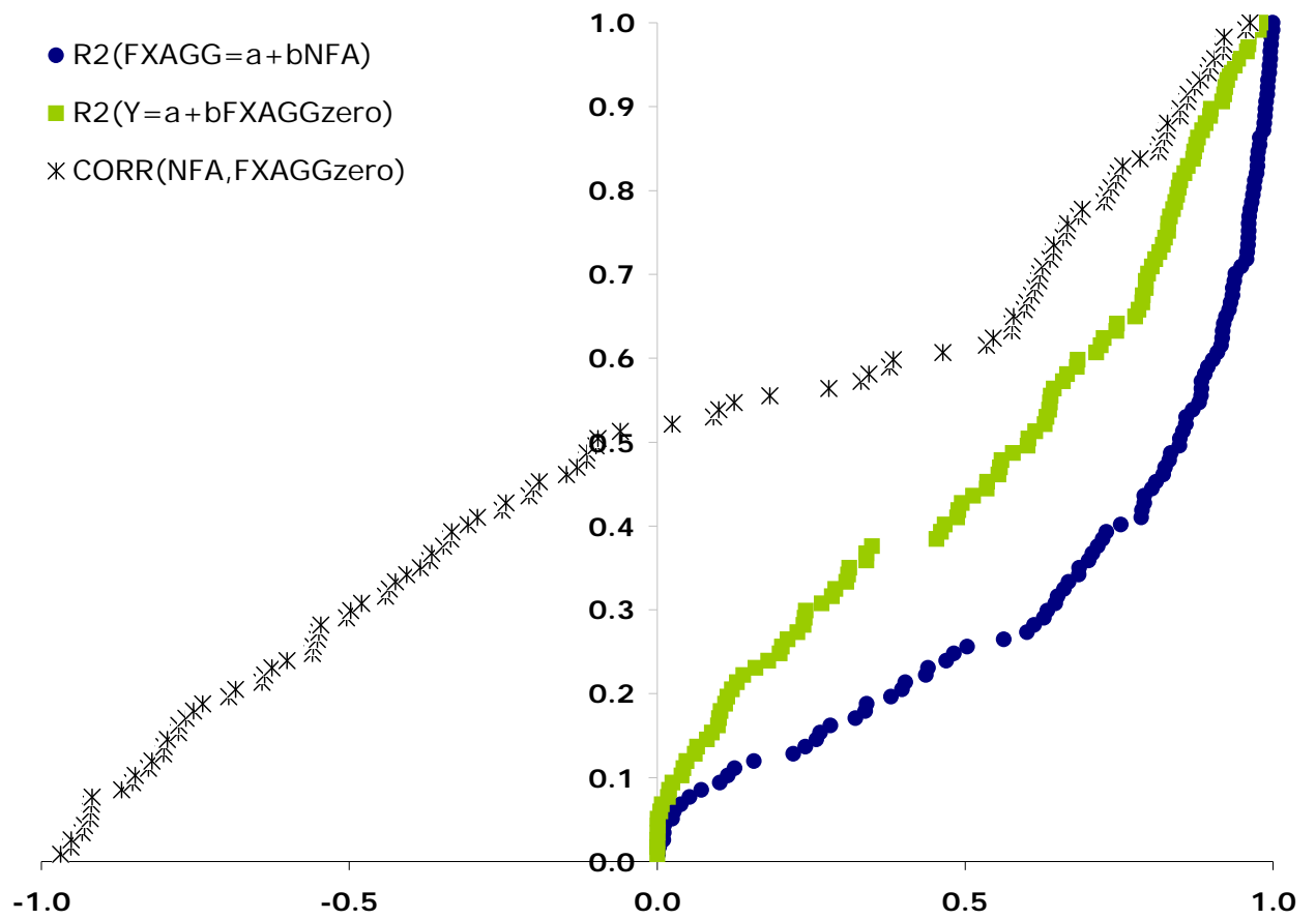
Figure 1: Decomposition: FX^{AGG} = NFA + FX^{AGG,zero} . (Net foreign assets scaled by A + L ). Cross-country Distribution of statistics.
