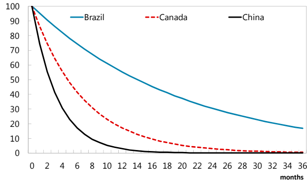
Figure 3. Path of Price Convergence: Response Functions (shock = 100, x axis in months)
