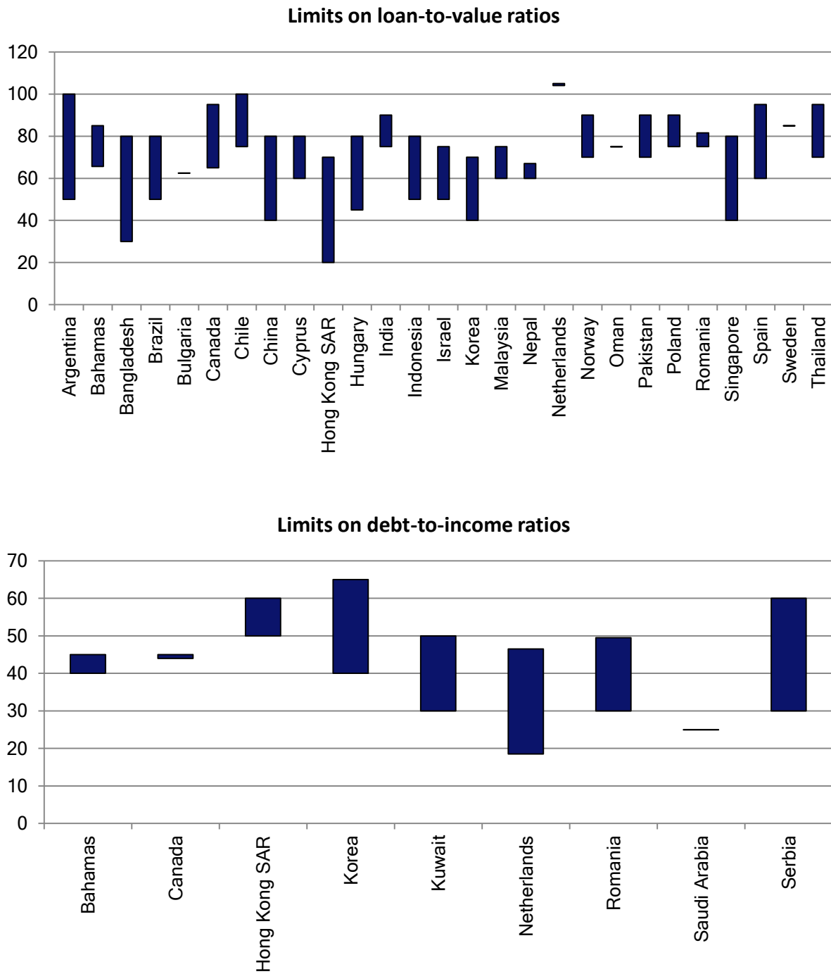
Figure 2. Range of Limits on LTV and DTI, 2013
