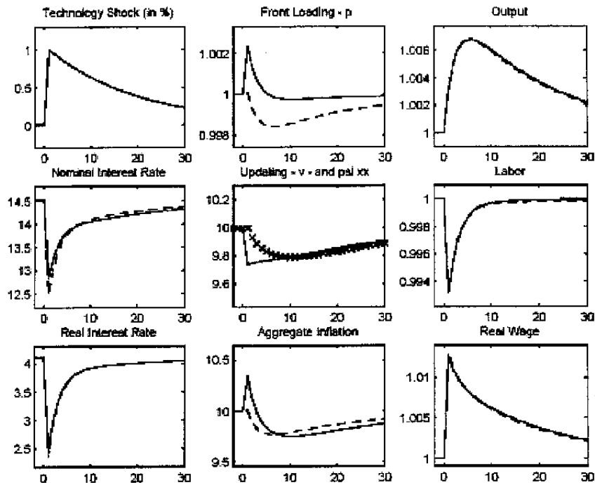
Figure 7. Technology Shock
