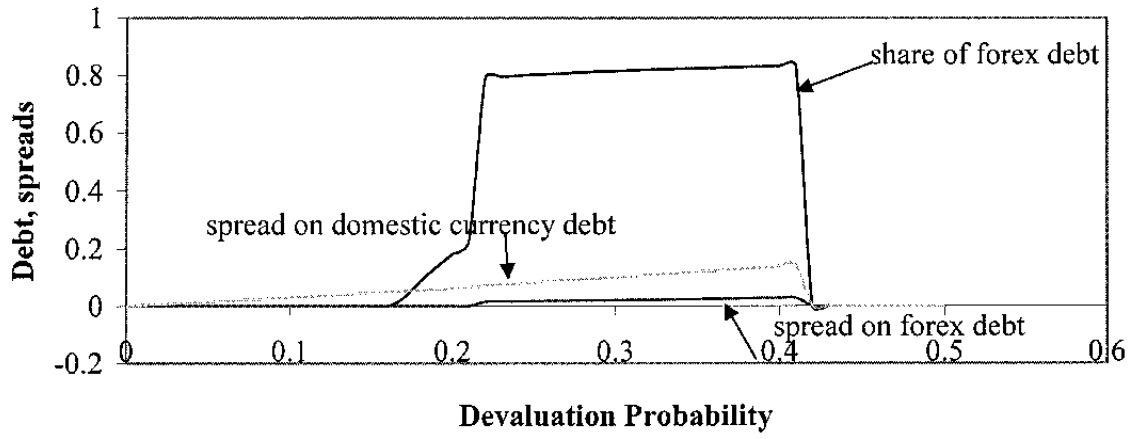
Figure 3. Devaluation Risk and Foreign Currency Debt
