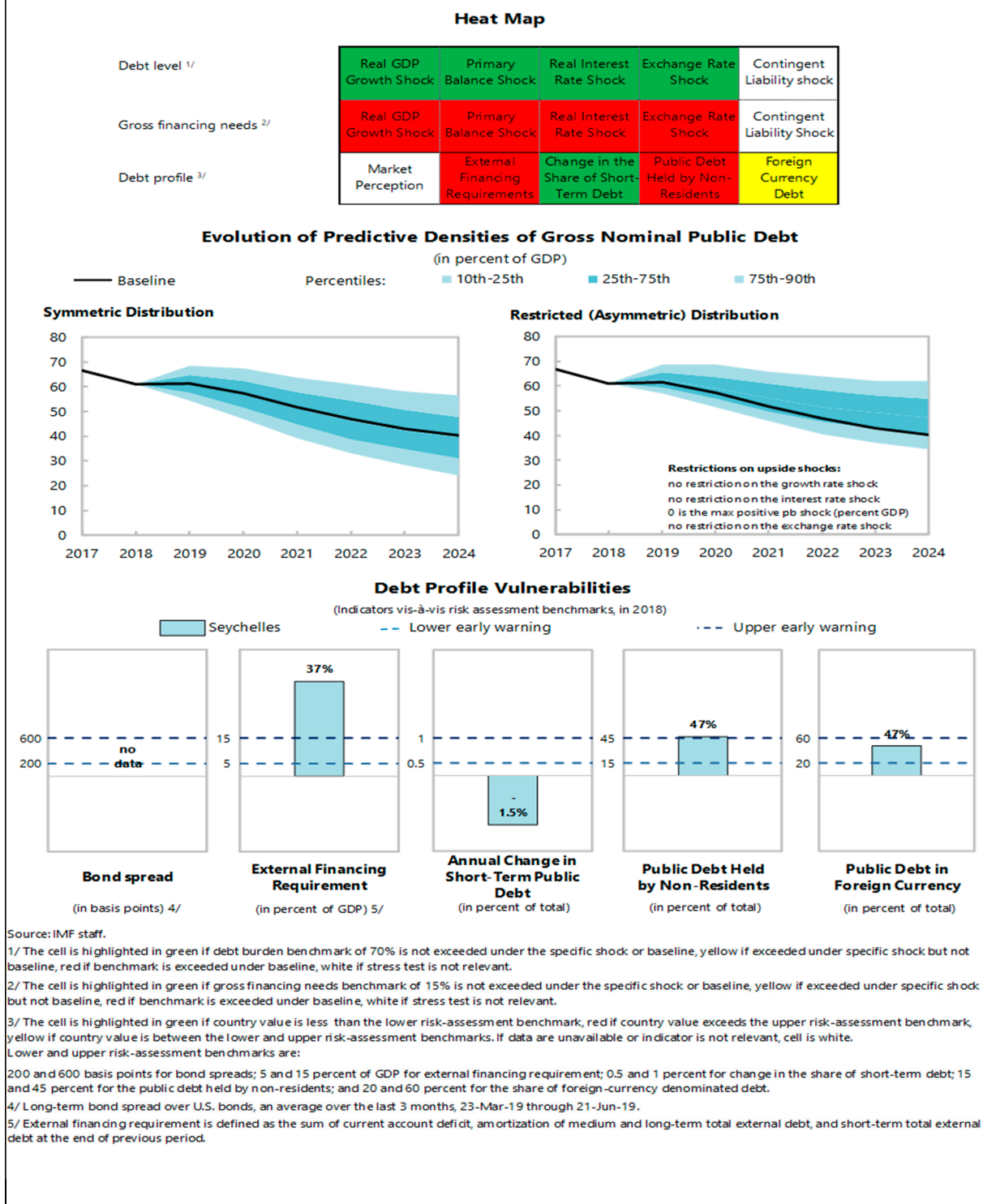
Figure 1. Seychelles: Public DSA Risk Assessment
