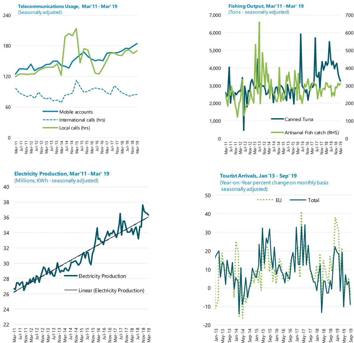
Figure 3. Seychelles: Monthly Indicators of Economic Activity
