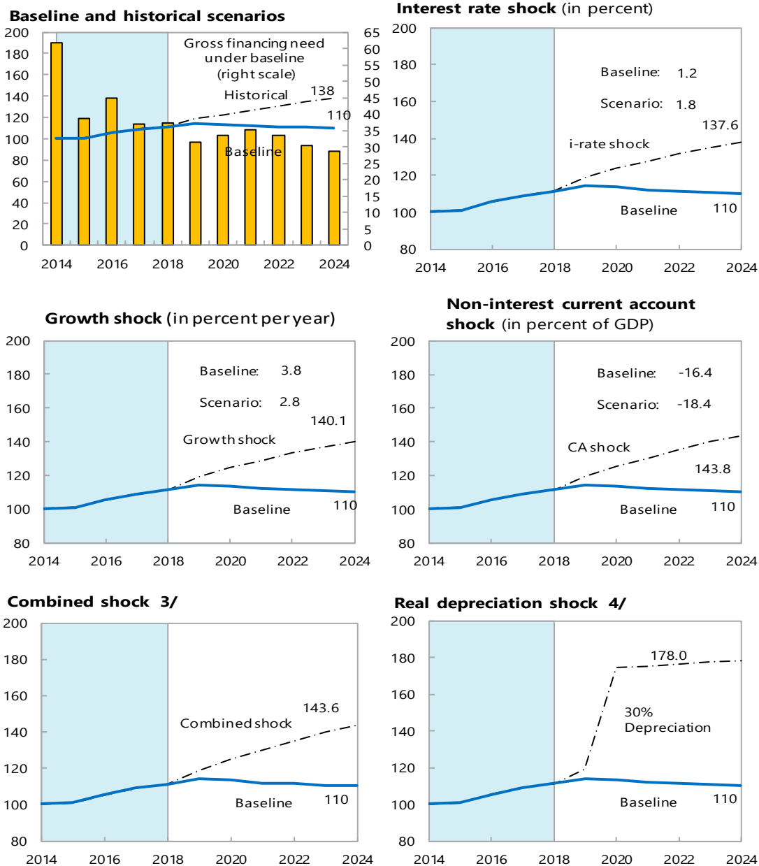
Figure 6. Seychelles: External Debt Sustainability: Bound Tests 1/ 2/
