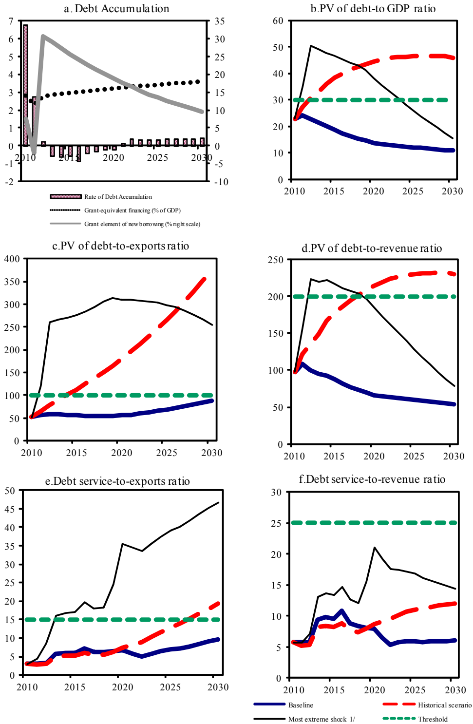
Figure 1. Chad: Indicators of Public and Publicly Guaranteed External Debt under Alternative Scenarios, 2010-2030 1/
