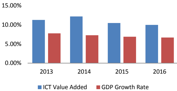
Chart 14 ICT Growth rate versus GDP growth rate for China
