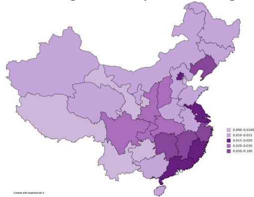
Chart 13 Regional development of the digital sectors
