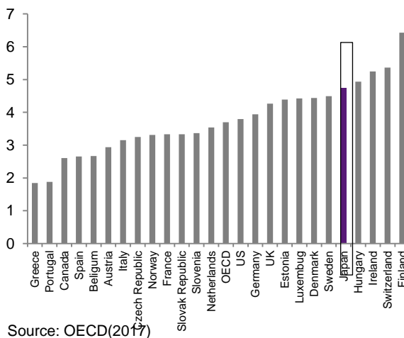
Chart 2 Employment in the ICT sector, % of total (2011 for OECD and 2010 for China)
